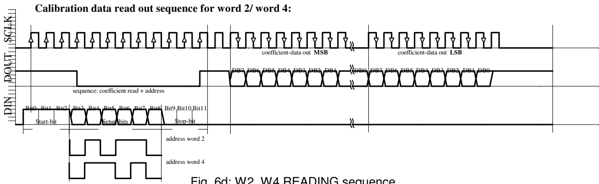
Fig. 6d: W2, W4 READING sequence
