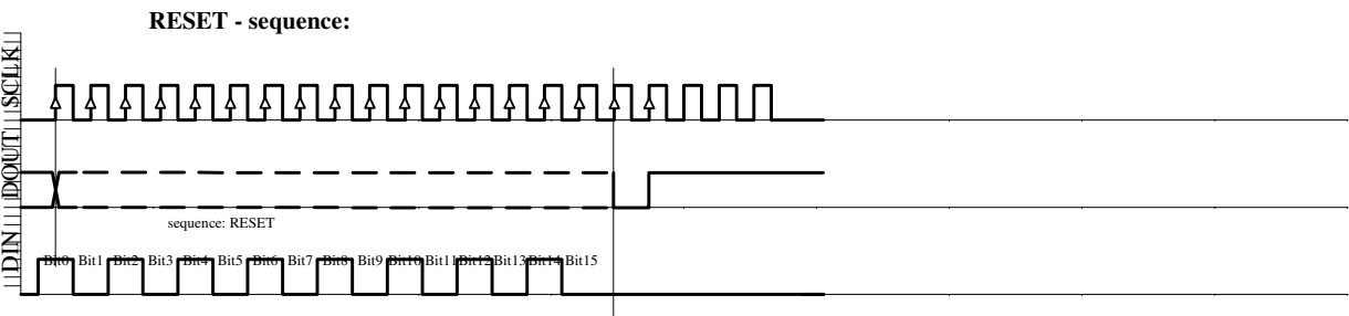
Fig. 6e: RESET sequence (21-Bit)
