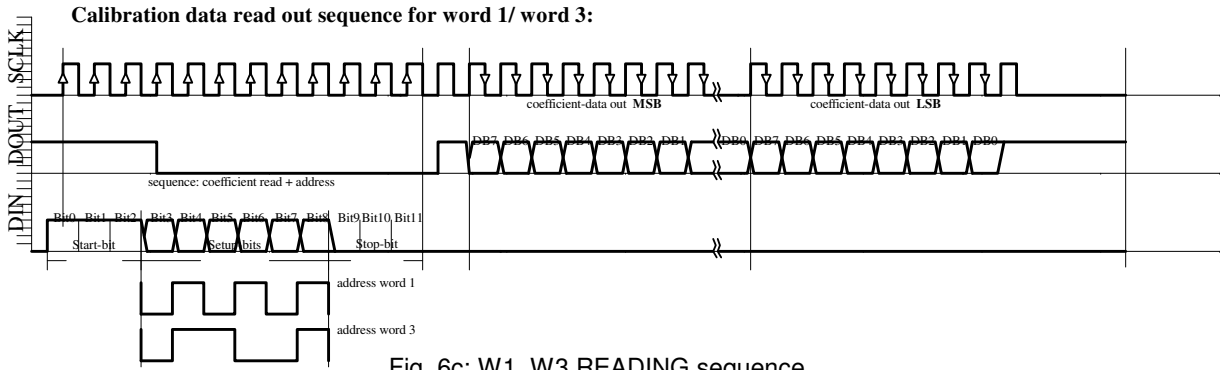
Fig. 6c: W1, W3 READING sequence
