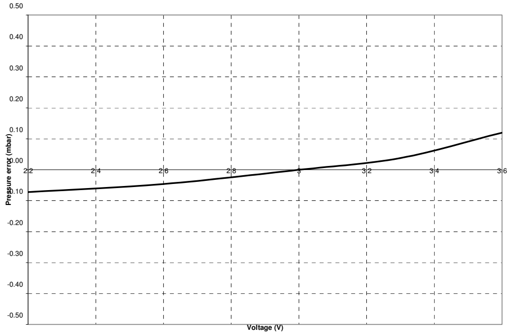
Pressure error vs supply voltage (typical)
