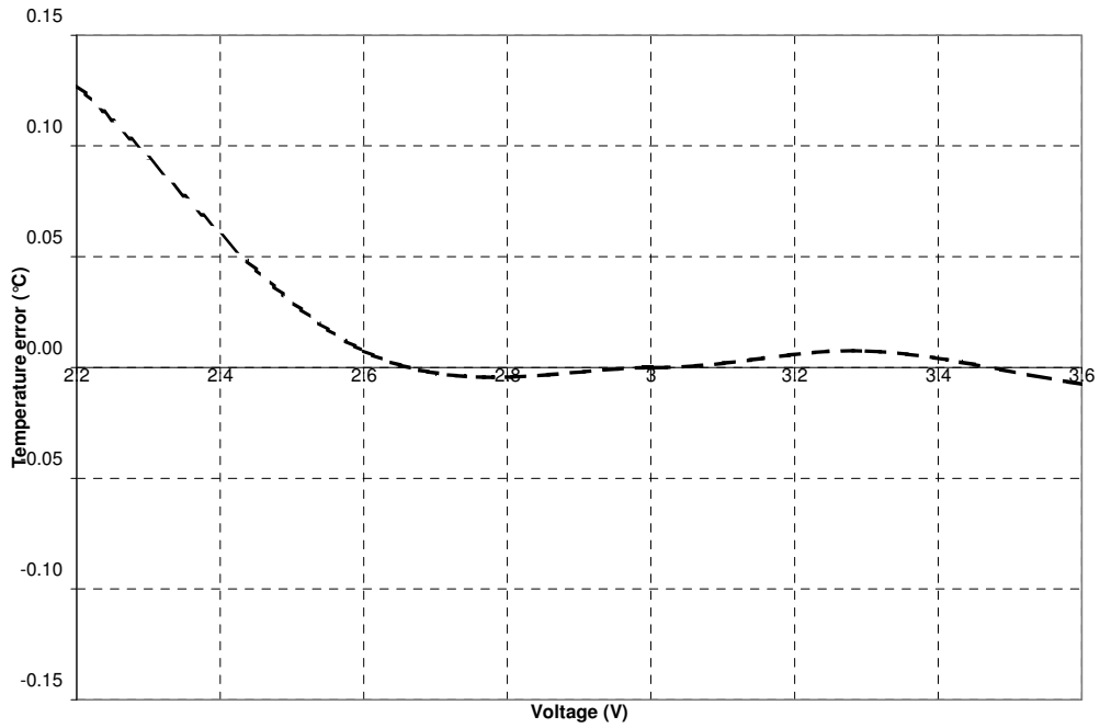
Temperature error vs supply voltage (typical)
