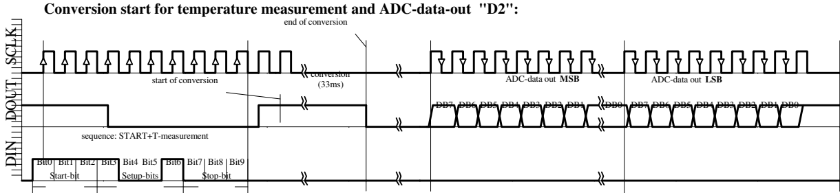
Fig. 6b: D2 ACQUISITION sequence
