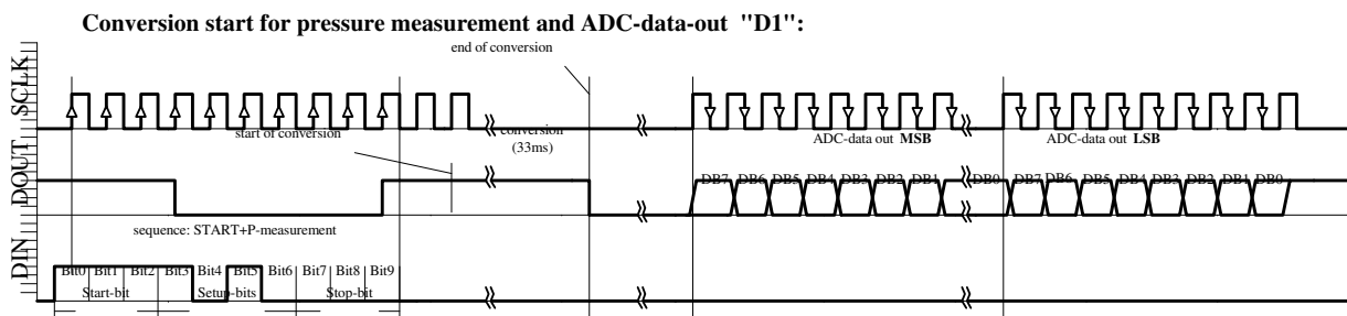
Fig. 6a: D1 ACQUISITION sequence
